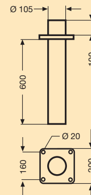
Maße in mm Erdrohr: Art. 3000 zu Kandelaber Art. 3020, 3024, 3025, 3027, 3032
